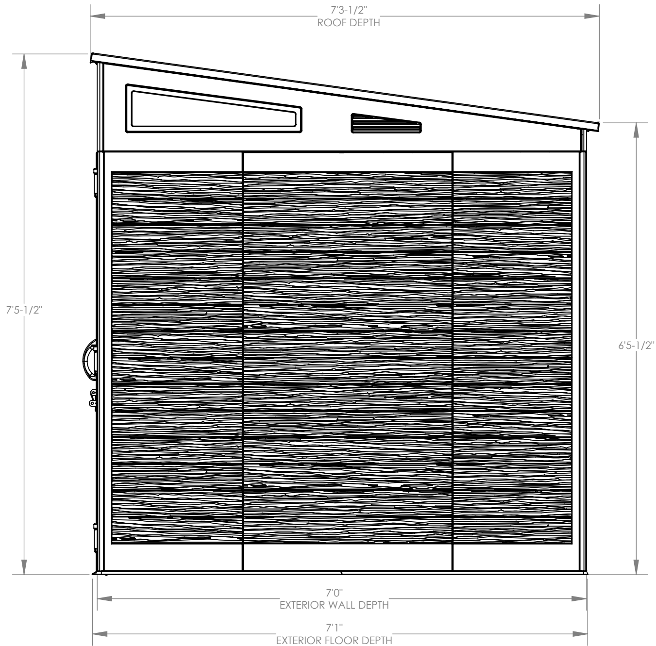
SIDE VIEW
