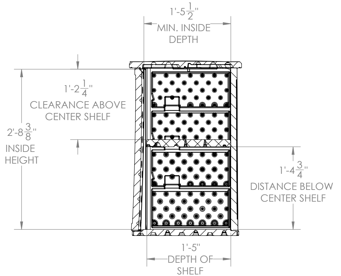
SIDE VIEW SECTION
